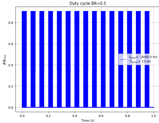
Fig. 4. Duty cycle for F_{\text{burst}} = 15 Hz and f_{\text{base}} = 2 kHz
