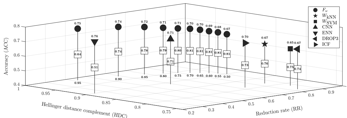
Fig. 2. Average performance results. They were calculated over the seven classifiers on the 40 datasets. Above each marker is shown the accuracy (ACC). The squared label shows the efficiency (E). The weight values ( w ) for the proposed approach F_w are shown at the bottom
