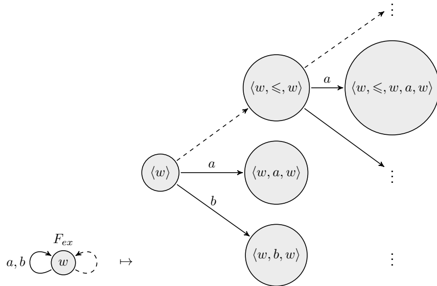
Fig. 3. Tree unraveling
