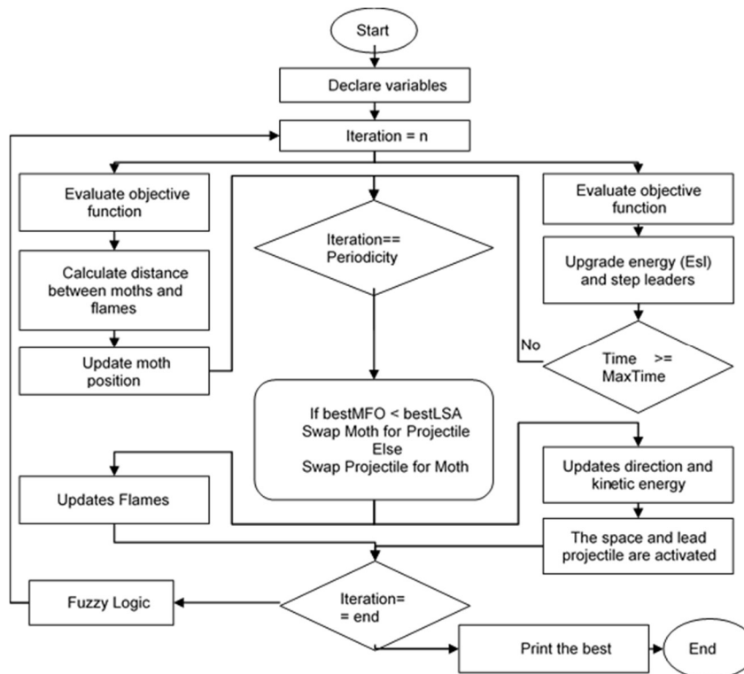
Fig. 3. Flowchart Lightning Search Algorithm
