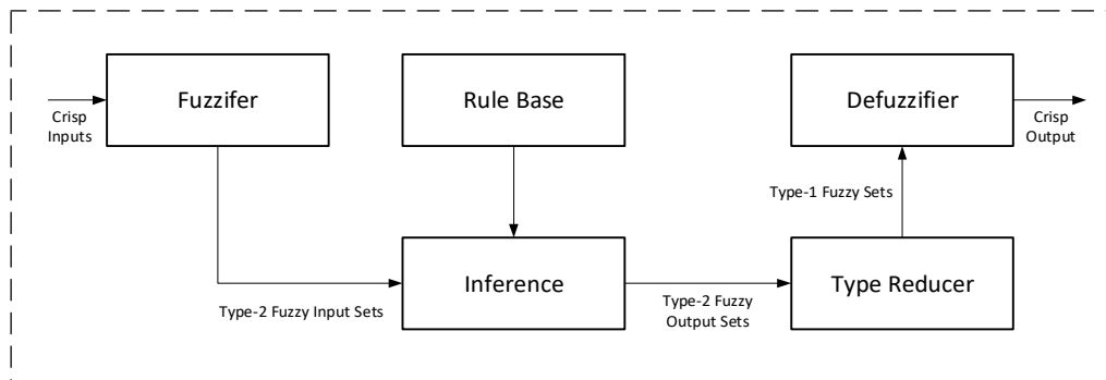
Fig. 6. Scheme of a Type-2 FLC
