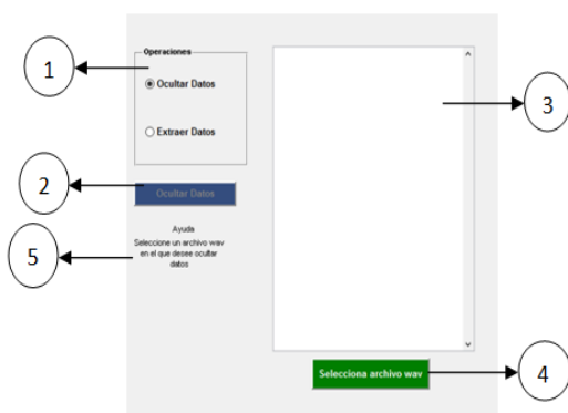
Fig. 5. Main Screen
