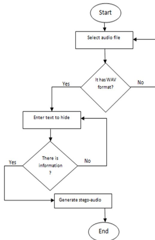
Fig. 3. Generating stego-audio
