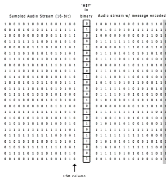
Fig. 2. Algorithm LSB
