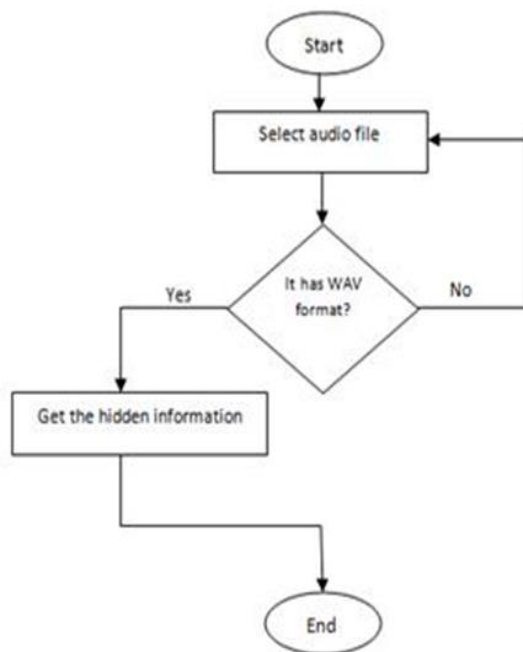
Fig. 4. Generating the hidden data
