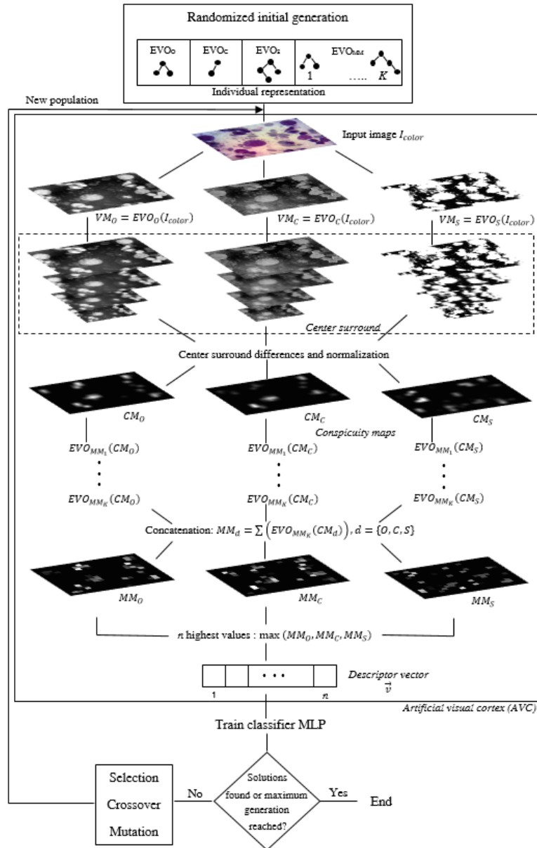
Fig. 1. General flowchart of the methodology
