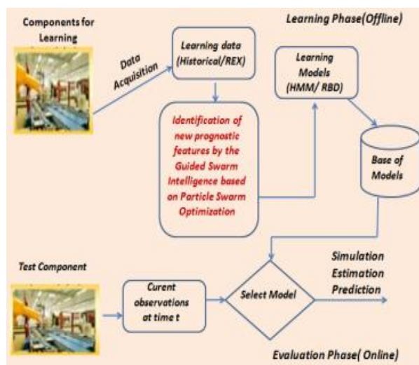
Fig. 8. Proposed methodology for prognosis with the identification of new prognostics features
