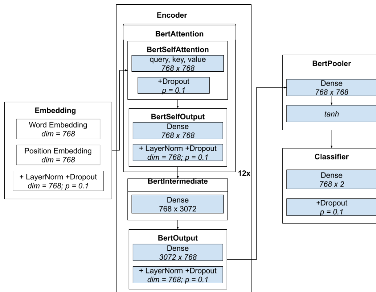
Fig. 1. BERT-En/Sp architecture
