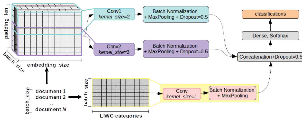
Fig. 2. CNN.glove+liwc architecture
