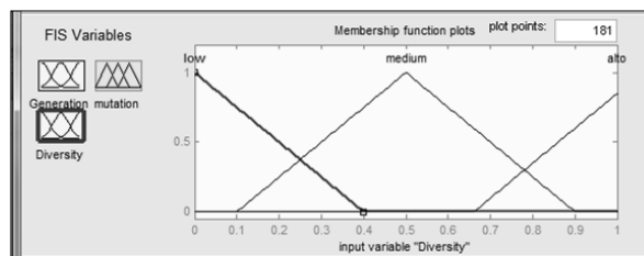
Fig. 4. Second Input (Diversity)
