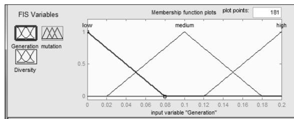
Fig. 3. First Input (Generation)
