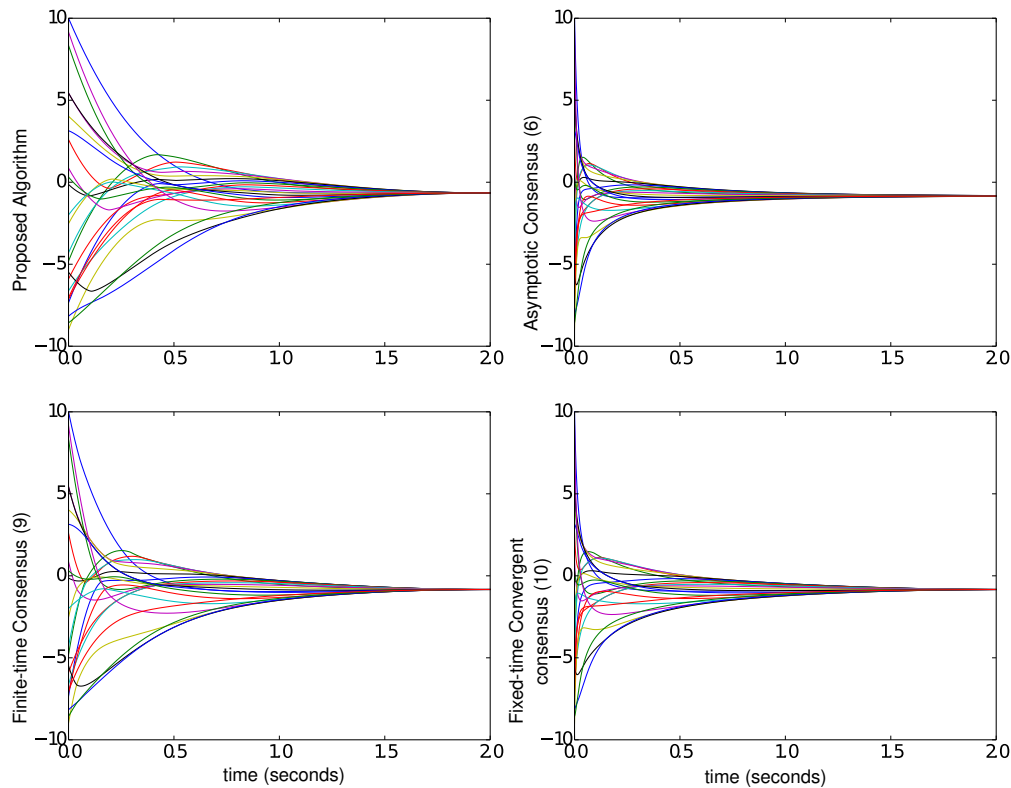
Fig. 1. Different consensus algorithms experimentally set for convergence to the consensus state approximately at 2 seconds under a cycle graph \mathcal{C}_{25} communication topology
