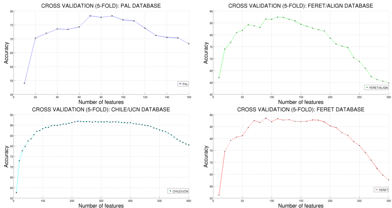
Fig. 4. Classification rate as a function of PCCA latent subspace dimensions
