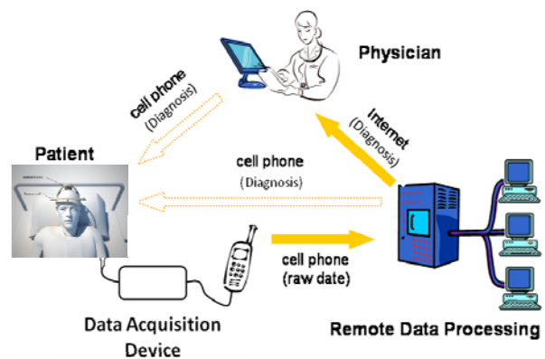
Fig 3. Schematic representation of the general concept for volumetric internal bleeding monitoring by electromagnetic induction phase shift spectroscopy. The figure shows the general design of the Data Acquisition Device to estimate the magnetic induction phase shift from the difference in phase between a reference voltage ( V_{ref} ) and a sensing voltage ( V_{ind} ) in an excitation and a sensing antenna respectively. The system includes the cell phone for data transmission by telecommunication lines for remote monitoring as well as the Advance Signal Processing unit. (Taken and adapted for academic purpose from Granot y. et al.) [26]
