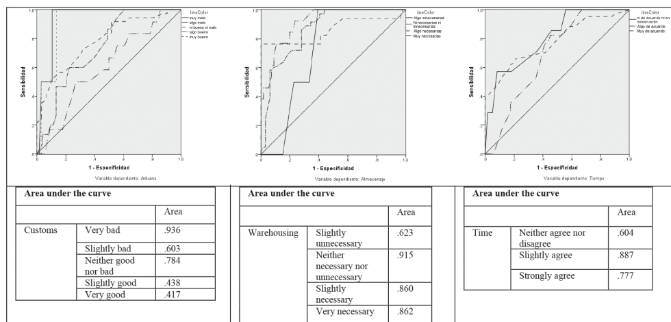
Figure 4. Forecast of satisfaction by variable for the variables: Customs, Warehousing and Time, ROC curve.
