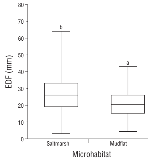
Figure 6. Entrance diameters of burrows measured in the field (EDF) in 2 microhabitats. Lines inside boxes are median values, box limits are standard errors of the mean, and error bars represent non-outlier ranges. Different letters above the boxes denote significant differences between groups of data (Tukey test after ANOVA, P < 0.05 ).
