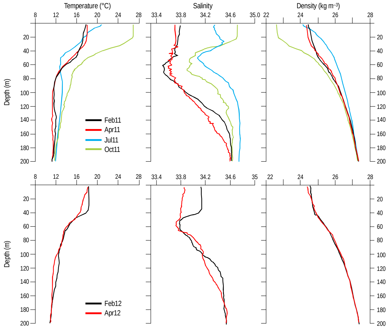
Figure 3. Average profiles of the thermohaline variables along the two most offshore transect lines (stations 5–68 and 4–67 in fig. 1c) for all cruises.
