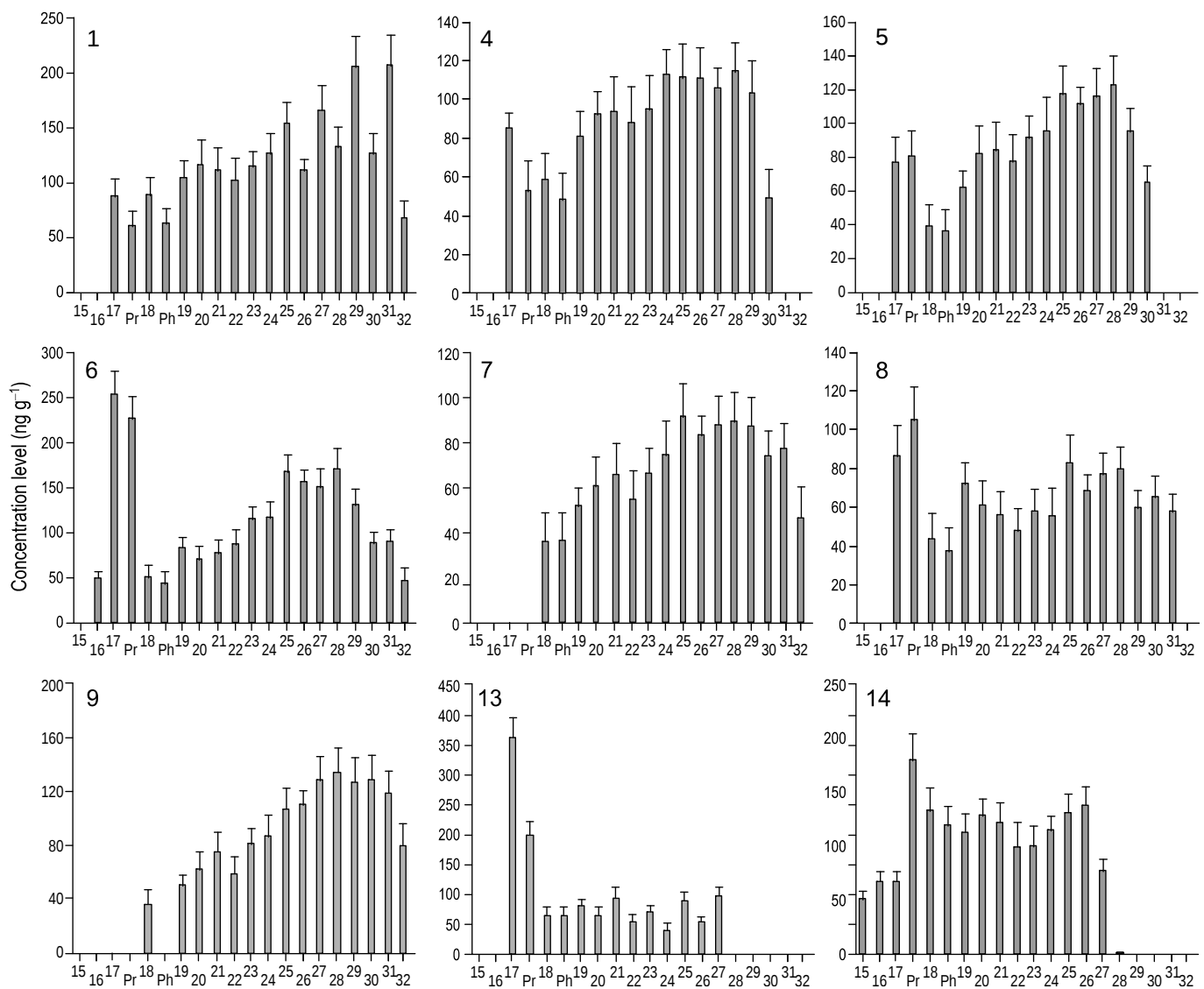
Figure 4. Typical n -alkane distributions from n - C_{15} to n - C_{32} detected in sediment samples collected at sites 1, 4, 5, 6, 7, 8, 9, 13, and 14 on the northeastern Havana seaboard. Pr: pristane; Ph: phytane.
