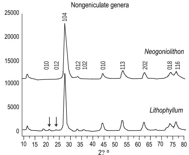
Figure 6. X-ray diffractograms of species of nongeniculate corallines. From the FTIR, as seen in figure 4, the most intense peak corresponds to the calcite (104) reflection and no amorphous phase is seen in any case. A third crystalline phase corresponding to the positions indicated by arrows was not identified. Almost all the calcite peaks show high asymmetry with a tail on the right side.
