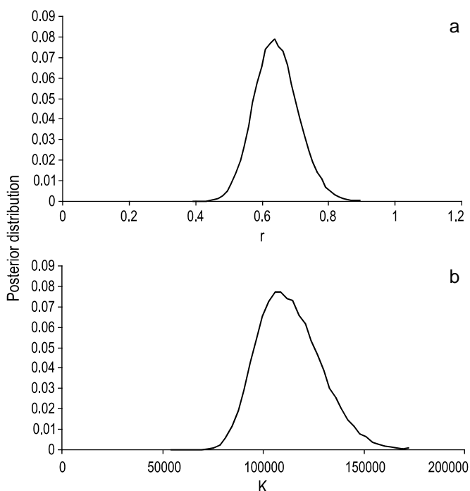
Figure 3. Posterior distributions for the Schaefer model parameters: (a) intrinsic growth rate and (b) carrying capacity.
