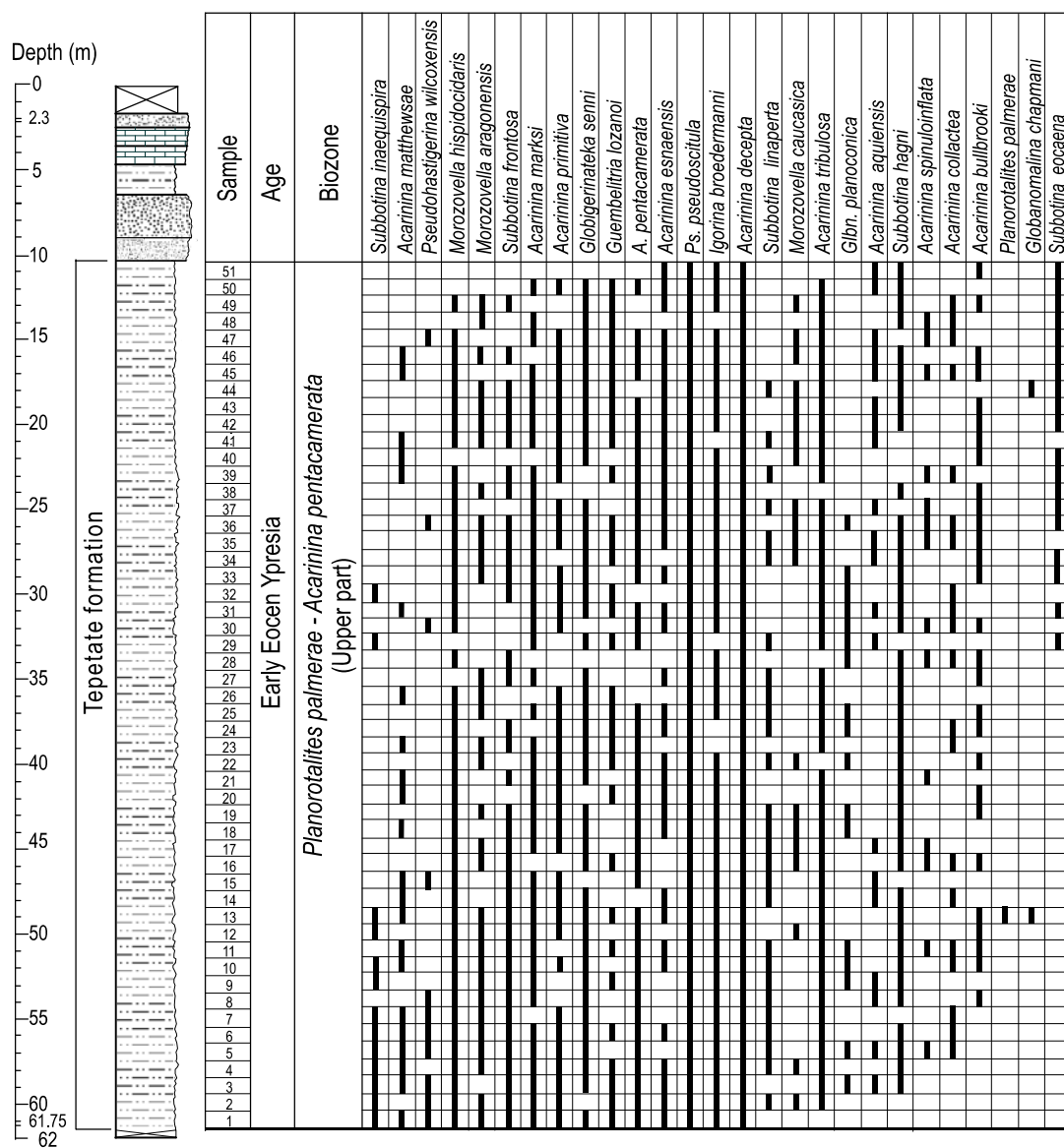
Figure 2. Distribution of planktonic foraminifers throughout the sedimentary column of Las Pocitas core.
