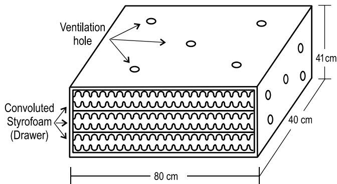
Figure 3. Design of the experimental transport box with convuluted (egg box) foam as principal material for egg protection.
