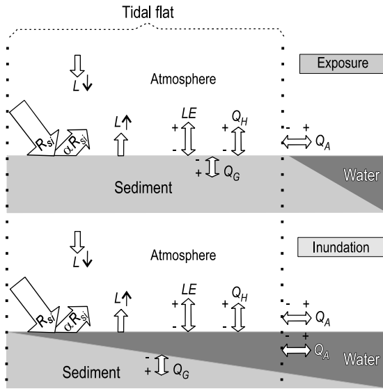
Figure 3. Scheme of the heat fluxes studied at the Puerto Cuatrerros tidal flat: R_{si} = incident solar radiation, \alpha R_{si} = reflected solar radiation, L_{\downarrow} = atmospheric longwave radiation, L_{\uparrow} = terrestrial longwave radiation, LE = latent heat flux, Q_H = sensible heat flux, Q_G = soil heat flux, and Q_A = advective heat flux.
