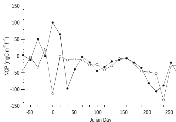
Figure 3. Time series of net community production (NCP, \text{mgC m}^{-2} \text{h}^{-1} ) in the Pontevedra Ria from October 1997 to October 1998 scaled from \text{NO}_3^- (●) and \text{PO}_4^{3-} (○) nutrient balances ( B_p , Eq. 5). A positive value implies net heterotrophy and a negative value, net autotrophy.
