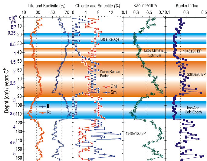
Figure 3. Vertical evolution of the clay mineral content, kaolin/illite ratio and Kubler index of illite crystallinity. Sediment layers, dated by ^{14}\text{C} are marked.
