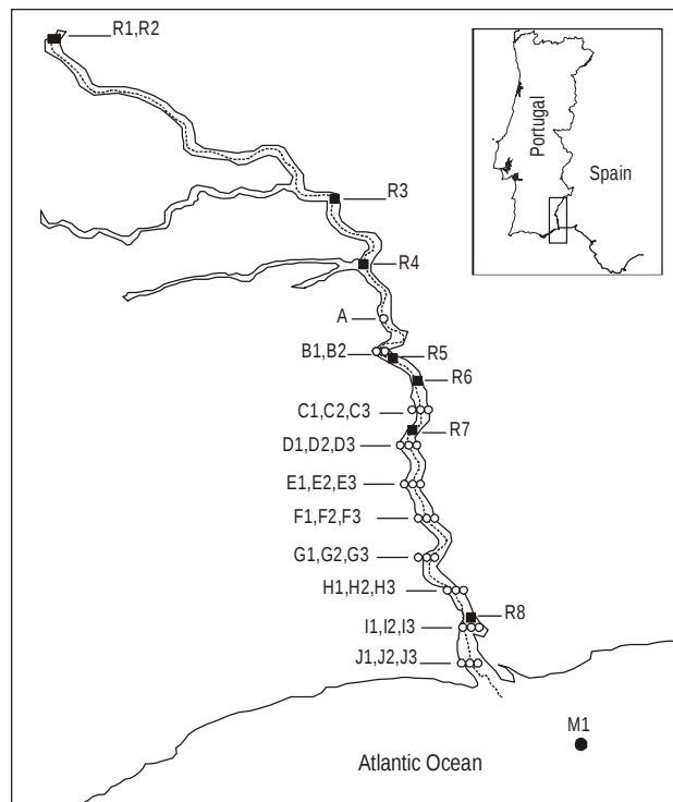
Figure 1. Location of the sampling stations in the Guadiana river-estuarine system: coarse material and freshly deposited particles transported by the river flood (■), surface sediments (○) and sediment core (●).
