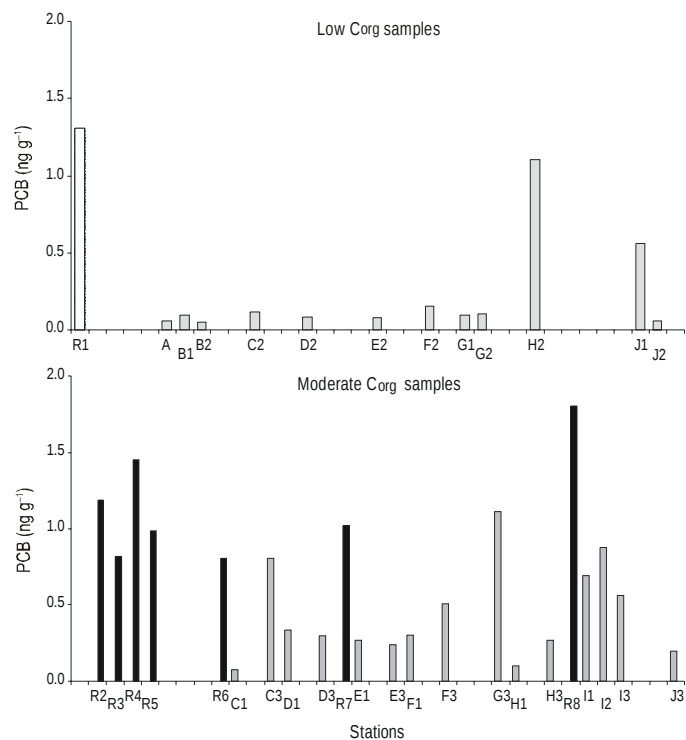
Figure 3. Longitudinal distributions of PCB ( \text{ng g}^{-1} ) in coarse material ( \square ) and freshly deposited particles transported by the river flood ( \blacksquare ) and in surface sediments ( \blacksquare ) from the Guadiana river-estuarine system with low and moderate organic carbon ( C_{org} ) content.
