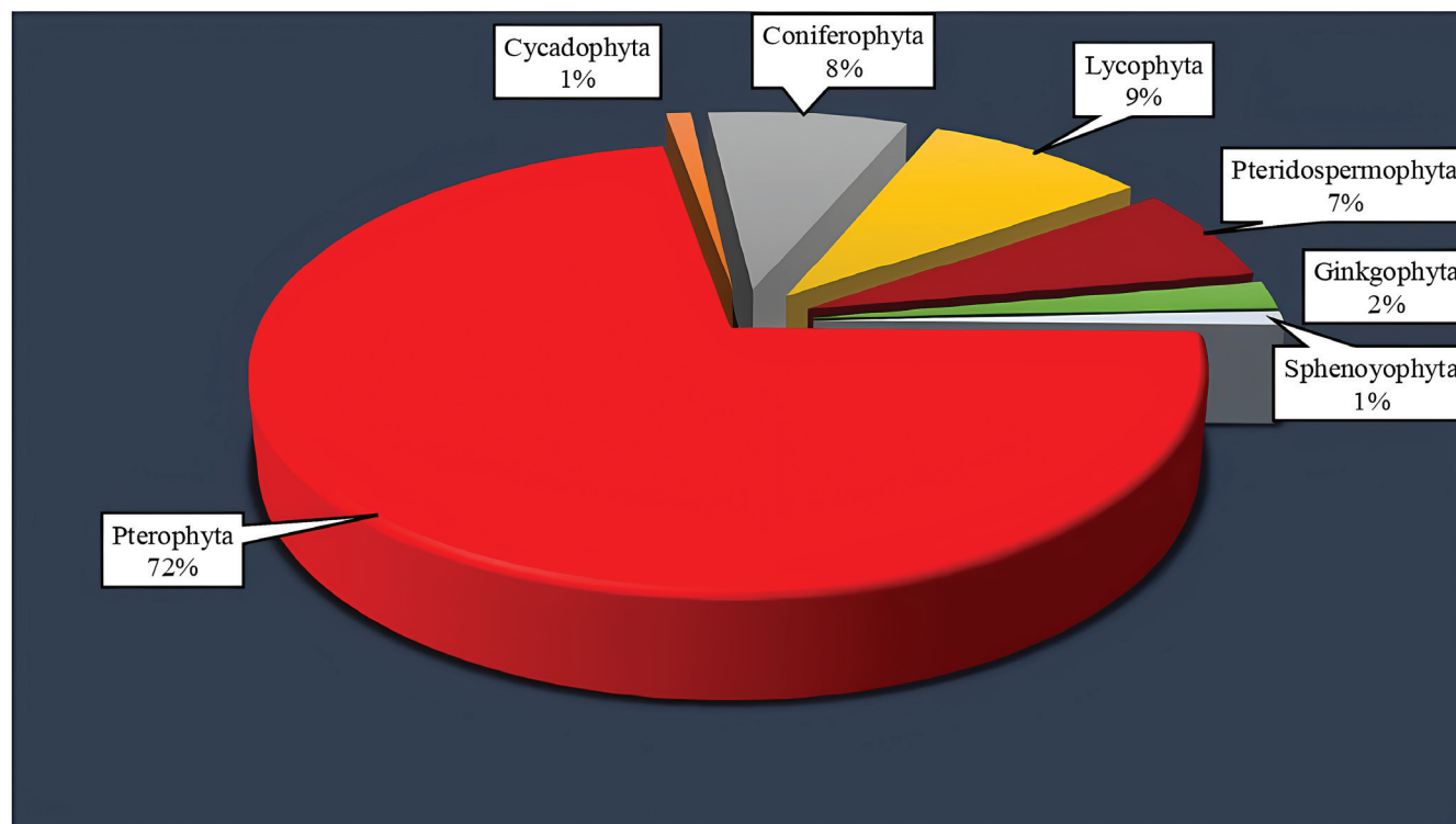
Figure 7 Diagram of abundance percentage of different groups of parent plants of miospores, Shemshak Formation, Namin stratigraphic section.
