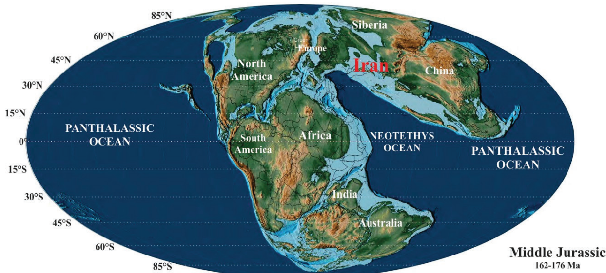
Figure 6 Paleogeographic Maps of the Middle Jurassic (modified after Robert et al. , 2014).
