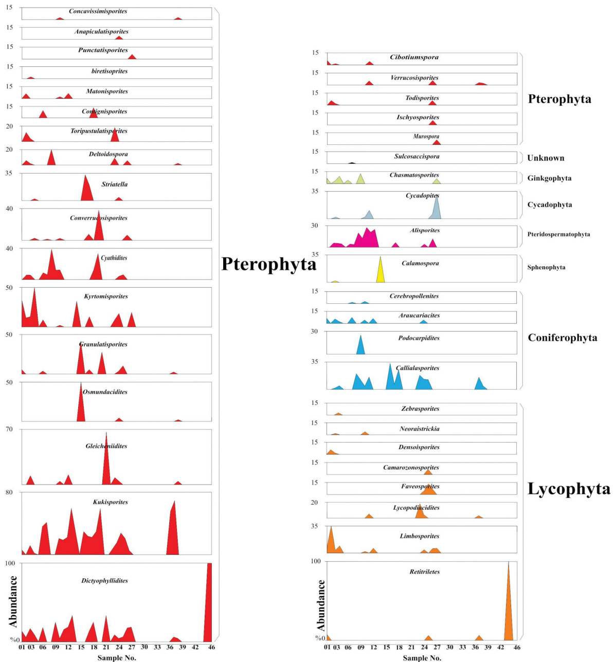
Figure 5 Abundance (percentage) of miospores of the Shemshak Formation at the Namin stratigraphic section.
