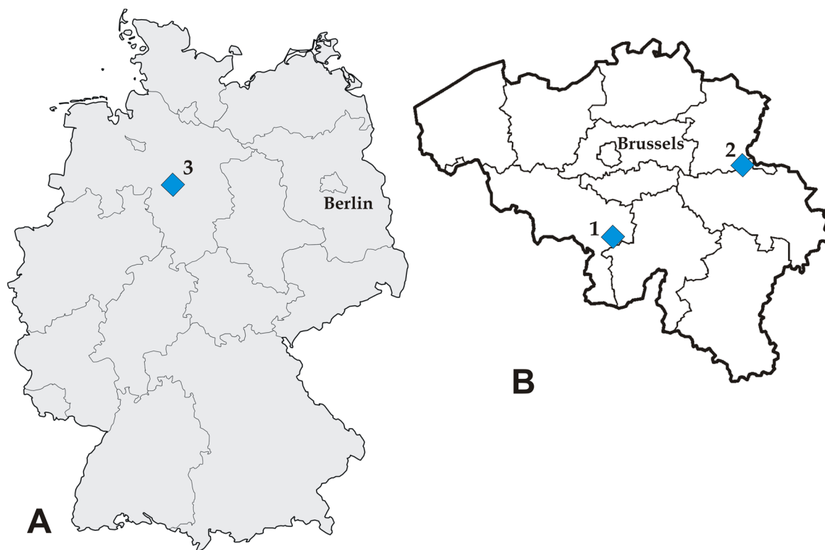
Figure 1 Schematic map of Germany (A) and Belgium (B), showing the provenance areas of material of Chomataster breizh sp. nov. and Nymphaster mudzborgh sp. nov. recorded herein: 1. Camp-à-Cayaux, near Spiennes, province of Hainaut (Mons Basin); 2. CBR-Romontbos quarry, Eben Emael-Bassenge, province of Liège (Liège-Limburg Basin); 3. Holcim-Höver and Teutonia (HeidelbergCement) quarries, Höver and Misburg-Anderten (Hannover area).
