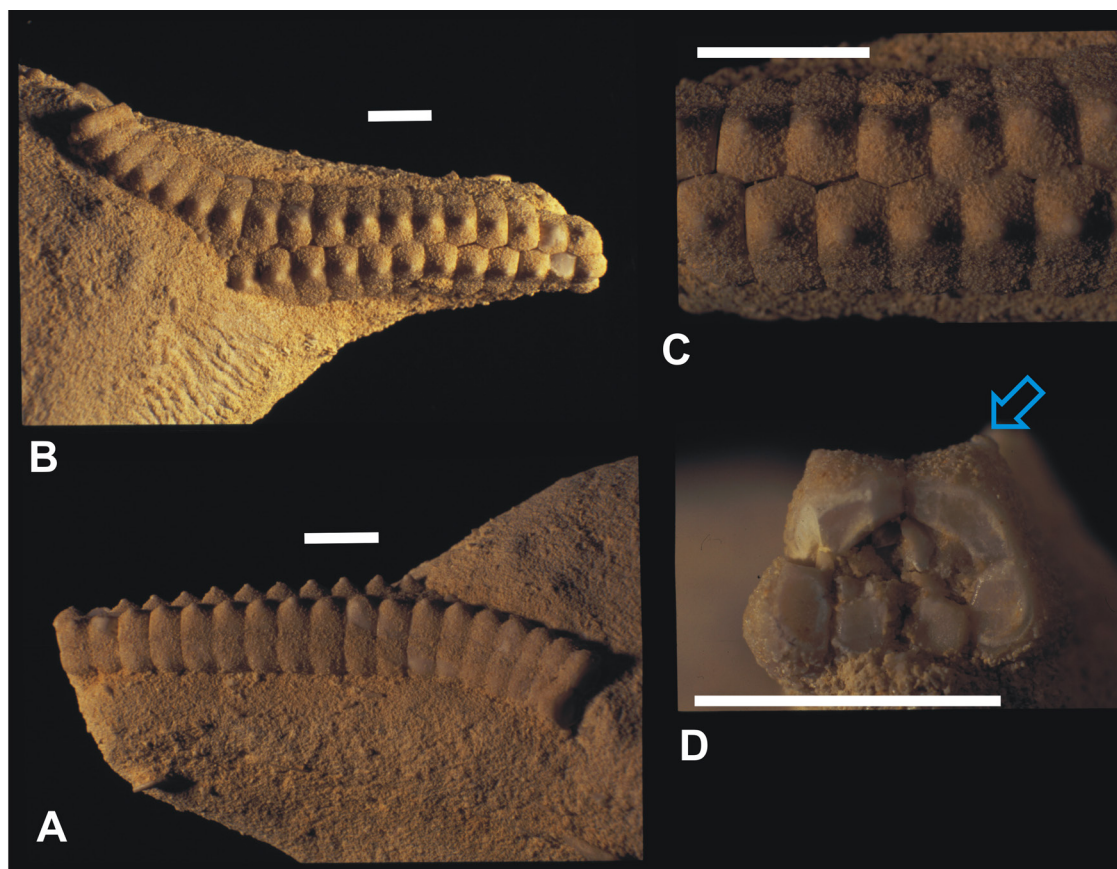
Figure 5 Chomataster breizh sp. nov. (paratype, NHMM van Rijsselt Collection, no. 100) from the lower Nekum Member (Maastricht Formation) at Eben Emael (CBR-Romontbos quarry). In A and B , the broad, evenly rounded interradius is seen; in C and D , the proximal portion of an arm is shown with regular alternation between superomarginals, and a cross-sectional view of the arm, with preserved superomarginal spine (arrow), stout and quadrangular adambulacrals and relatively sturdy and small ambulacrals. Scale bars equal 10 mm.
