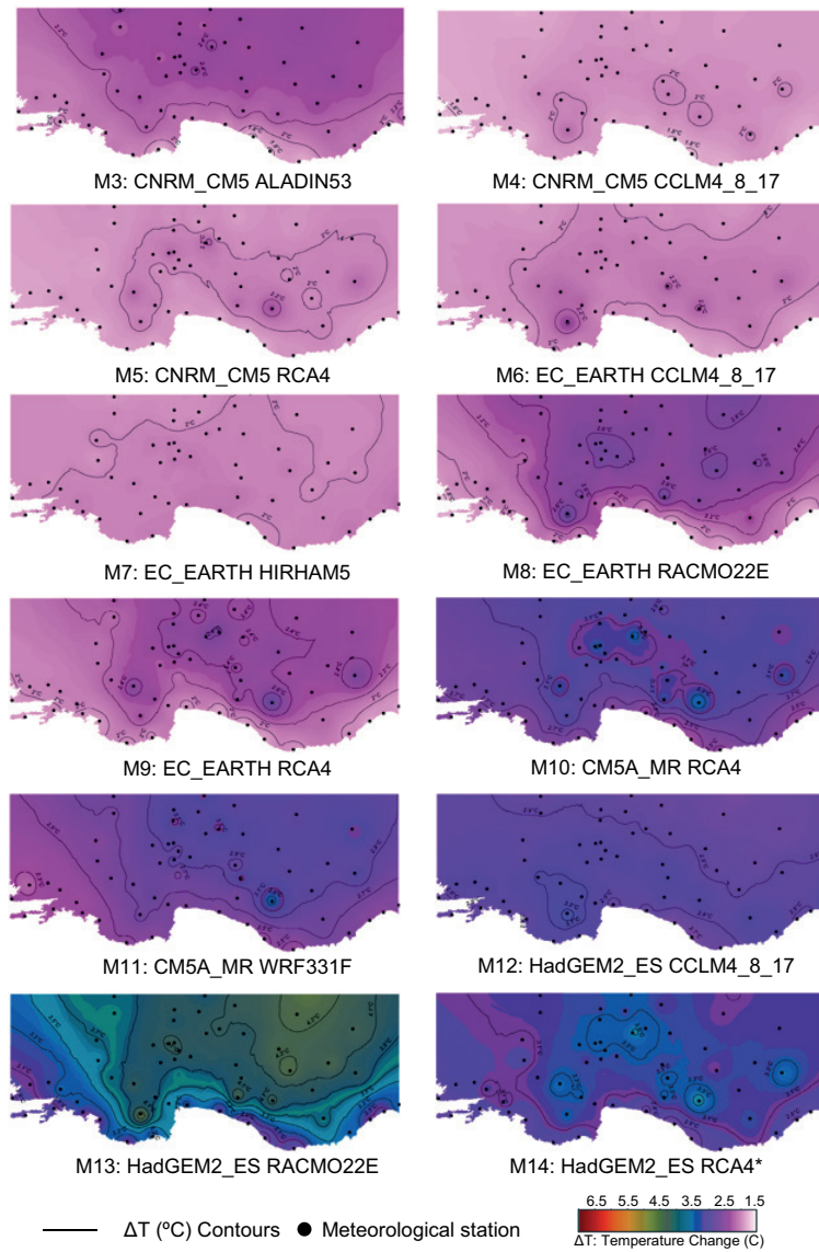
Fig. S11. Long-term temperature change projections (RCP4.5) ( \Delta T_{annual} [°C]) for models M3 through M14. All changes are verified to be statistically significant at the 95% confidence level. (*Best performing CORDEX model for the study area).
