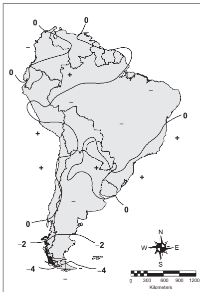
Fig. 10. Cold period's model. Type I (in mb).
