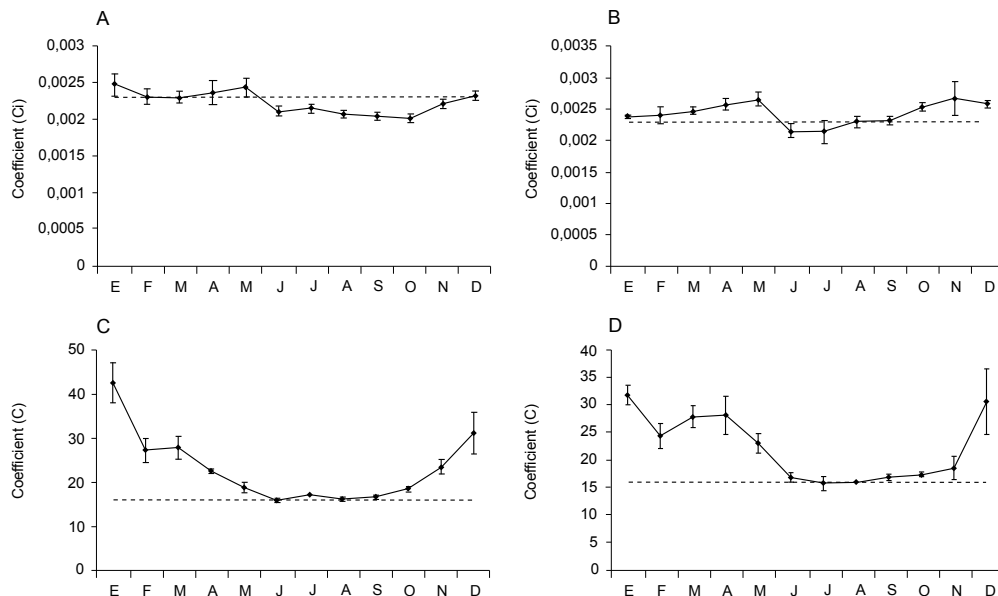
Fig. 4. Monthly values of the constants of adjusted HM and adjusted TM. Inland (A and C) and coastal (B and D) meteorological stations with its original values (---).
