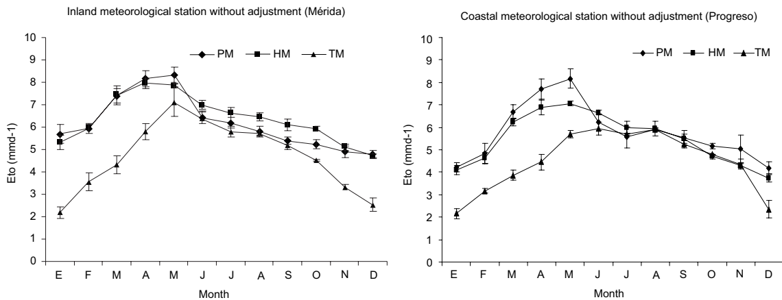
Fig. 3. Monthly averages of ETo without adjustment for the time period 2001-2003 in the tropical subhumid climate station (Mérida) and in the semiarid climate station (Progreso).
