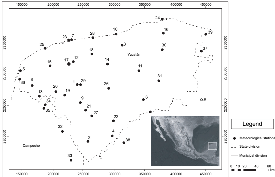
Fig. 1. Localization of the meteorological stations considered in this study.
