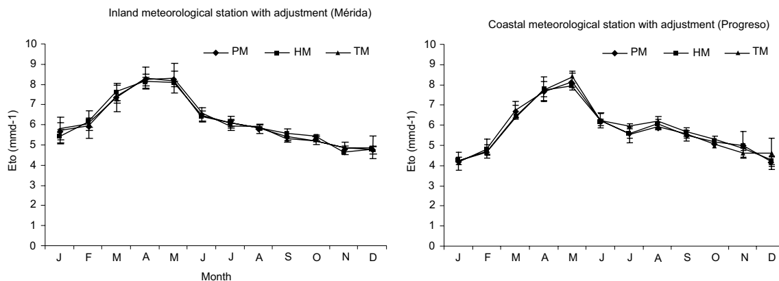
Fig. 6. Monthly mean estimation of ETo with adjustment for the period 2001-2003 in the tropical subhumid climate station (Mérida) and in the semiarid climate station (Progreso).
