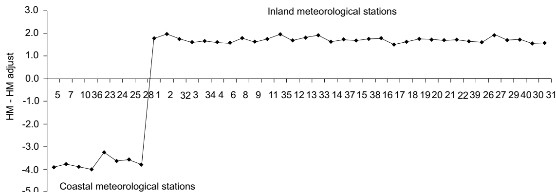
Fig. 7. Annual differences using adjusted and non adjusted Eto values with HM from all meteorological stations
