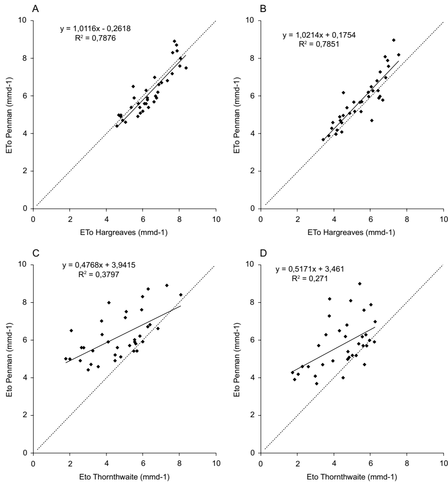
Fig. 2. Regression models of ETo for Penman (PM) vs Thornthwaite (TM) without adjustment and Penman (PM) vs Hargreaves (HM) without adjustment for the meteorological stations of Mérida (A and C) and Progreso (B and D).
