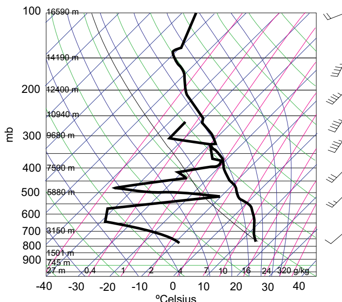
Fig. 4. Radiosonde from México City international Airport (6:00, April 2007). Plot shows vertical dew point profile (left) and temperature profile (right). Temperature line does not show any inversion layer from surface up to 600 mb (Source: University of Wyoming).
