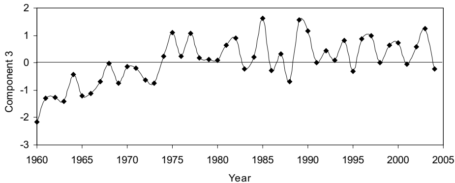
Fig. 3. Time series plot of standardized scores for the component related to the moderately large extreme events over the period 1960-2004.
