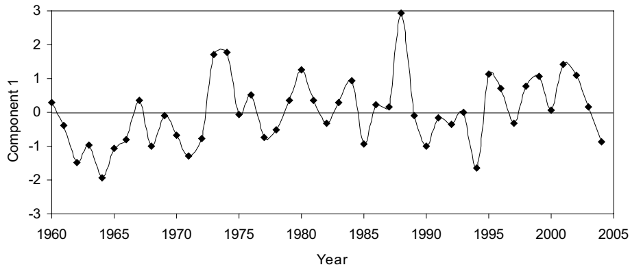
Fig. 2. Time series plot of standardized scores for the component related to the largest of the extreme events over the period 1960-2004.
