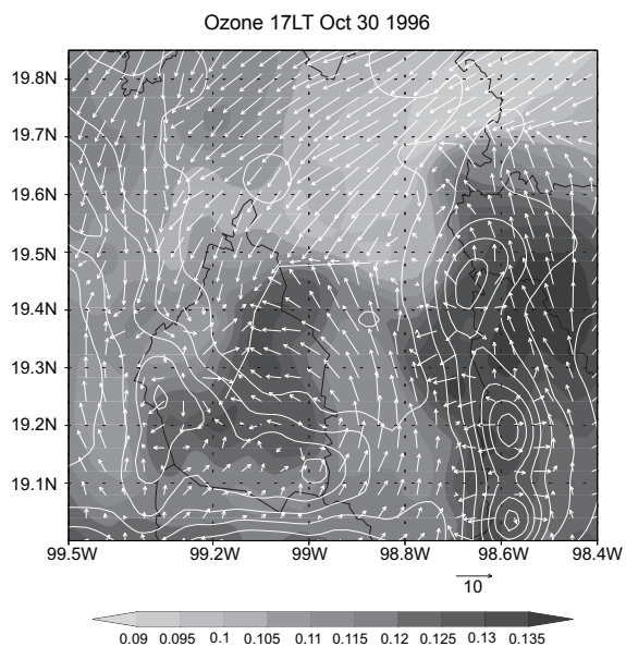
Fig. 9. In a) Surface wind fields in \text{ms}^{-1} and ozone mixing ratios in ppm, for October 30, 1996, 17:00 LT. The white lines signal the position of a confluence. Highest ozone mixing ratios accumulate around the confluence line in the north and southwest of México City. In b), the same information but for January 29, 2001, 13:00 LT. Highest ozone mixing ratios accumulate around the confluence line. (From Jazcilevich, 2005).
