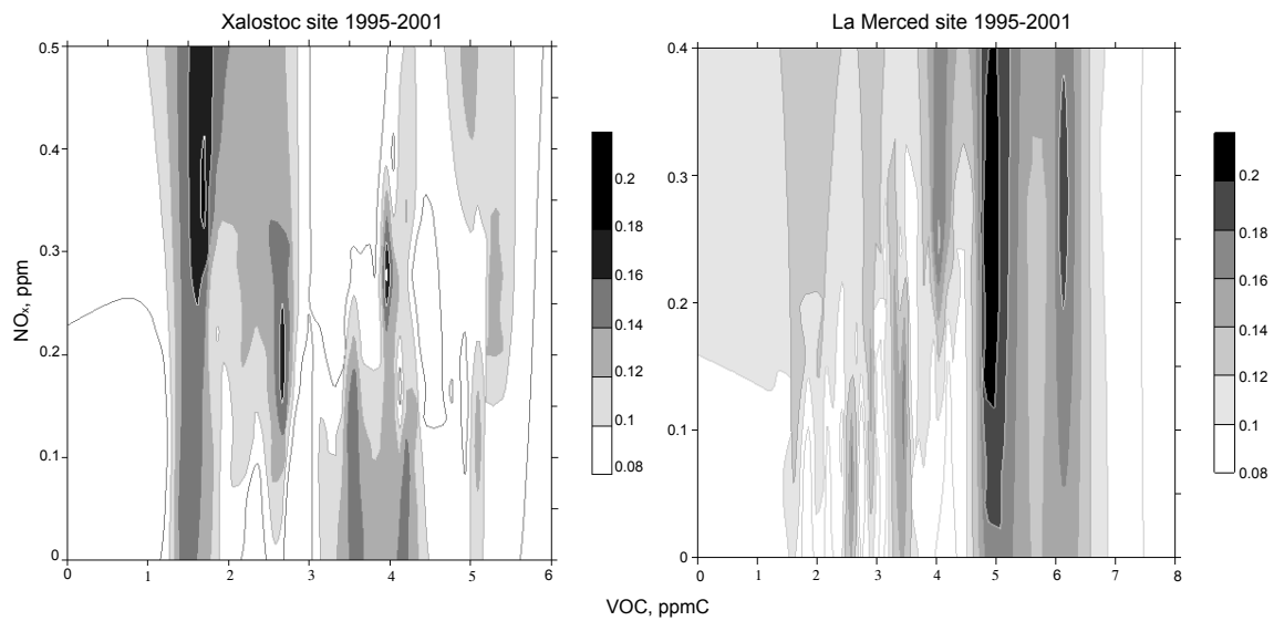
Fig. 7. Ozone isopleths for La Merced site, 0600 to 0900 measurements from 1995-2001.
