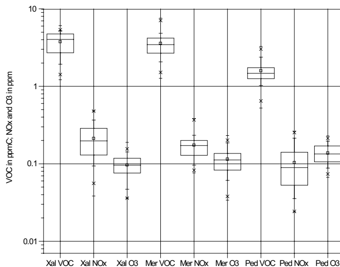
Fig. 2. VOC, \text{NO}_x , and maximum concentrations of \text{O}_3 for Xalostoc, (Xal), Merced (Mer), and Pedregal (Ped) from 1995 to 2001.
