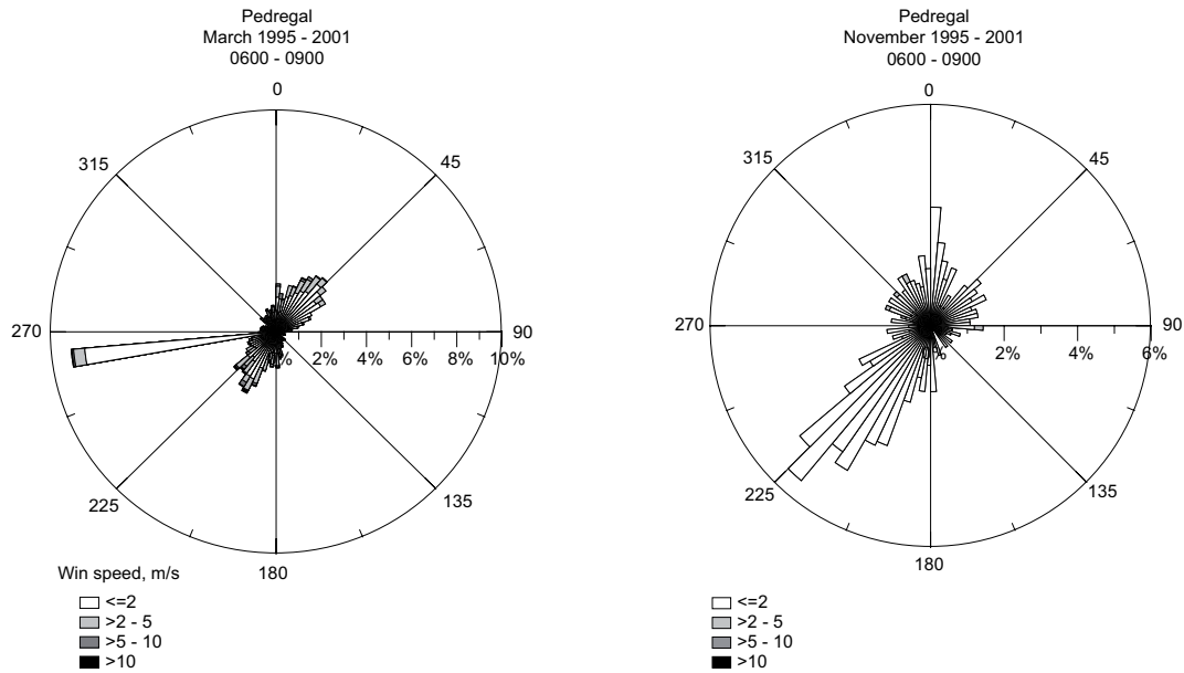
Fig. 5. Pedregal wind roses for March and November 1995-2001.
