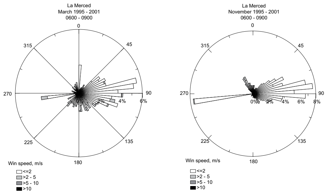
Fig. 4. La Merced wind roses for March and November 1995-2001.
