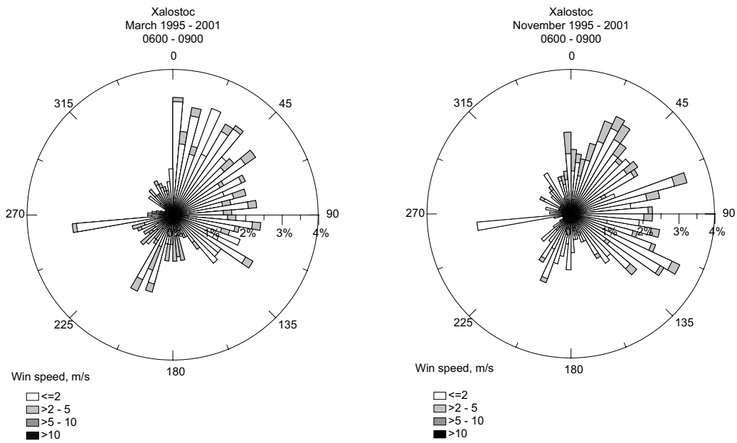
Fig. 3. Xalostoc wind roses for March and November 1995-2001.
