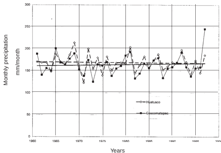
Fig. 2. Yearly means of total monthly precipitation, Huatusco and Coscomatepec.
