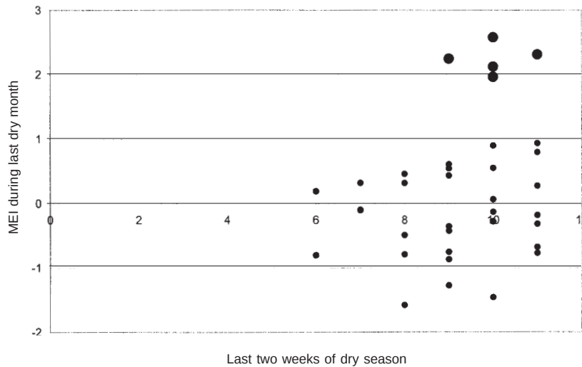
Fig. 10. MEI vs. last two weeks of dry season (1983, 1987, 1992, 1993 and 1997: years of strong ENSO are big dots).
