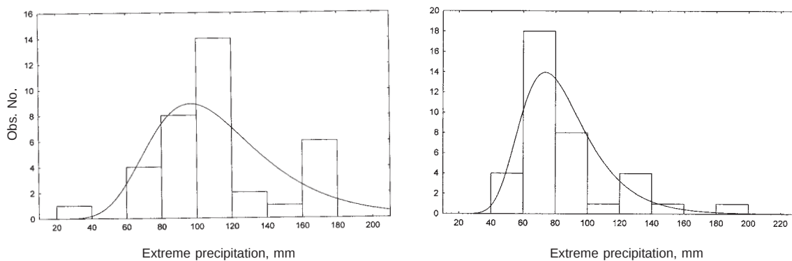
Fig. 5. Gumbel distributions for Huatusco (left) and Coscomatepec (right) fitted to extreme yearly values of 37 years of data. Notice the small secondary maximum to the right of the histograms.
