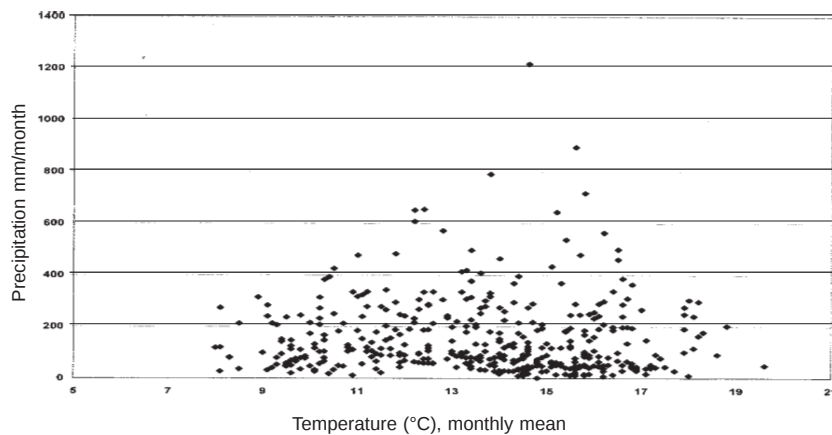
Fig. 8. Monthly cumulated precipitation vs. monthly mean temperature Atzalán, Ver.).
