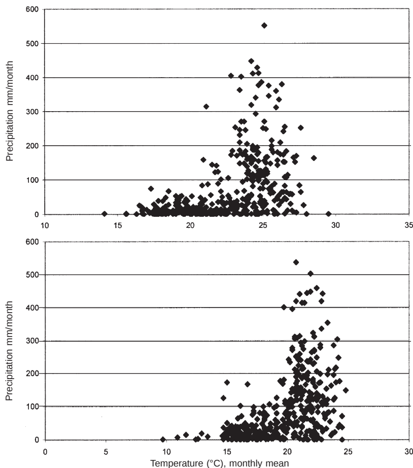
Fig. 6. Monthly-cumulated precipitation vs monthly mean temperature (Actopan, Ver.).
