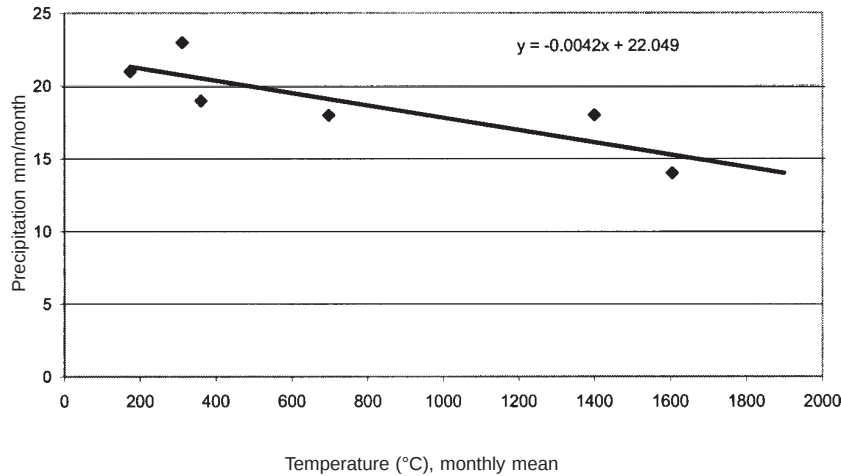
Fig. 9. Threshold of temperature for precipitation above 100 mm/month vs. altitude of the corresponding station.
