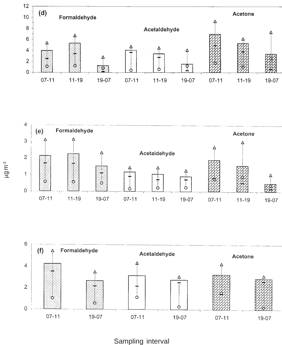
Fig. 2. Diurnal carbonyl mean concentration variations in each sampling site: (a) and (b) Rancho Viejo, first and second sampling, respectively; (c) and (d) Temascaltepec, first and second sampling, respectively; (e), (f), and (g) Monte Pío, Cuetzalan, and the Biology Station, respectively. Columns indicate mean values; dashes-minimum values; triangles-maximum values; circles-standard deviation.
