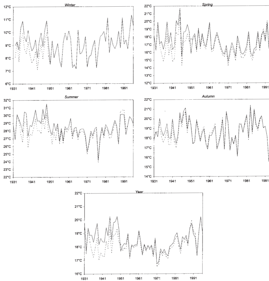
Fig. 2a. Differences between homogenized (continous line) and non-homogenized series (dashed line) of seasonal and annual maximum temperatures in Zamora (Spain).
