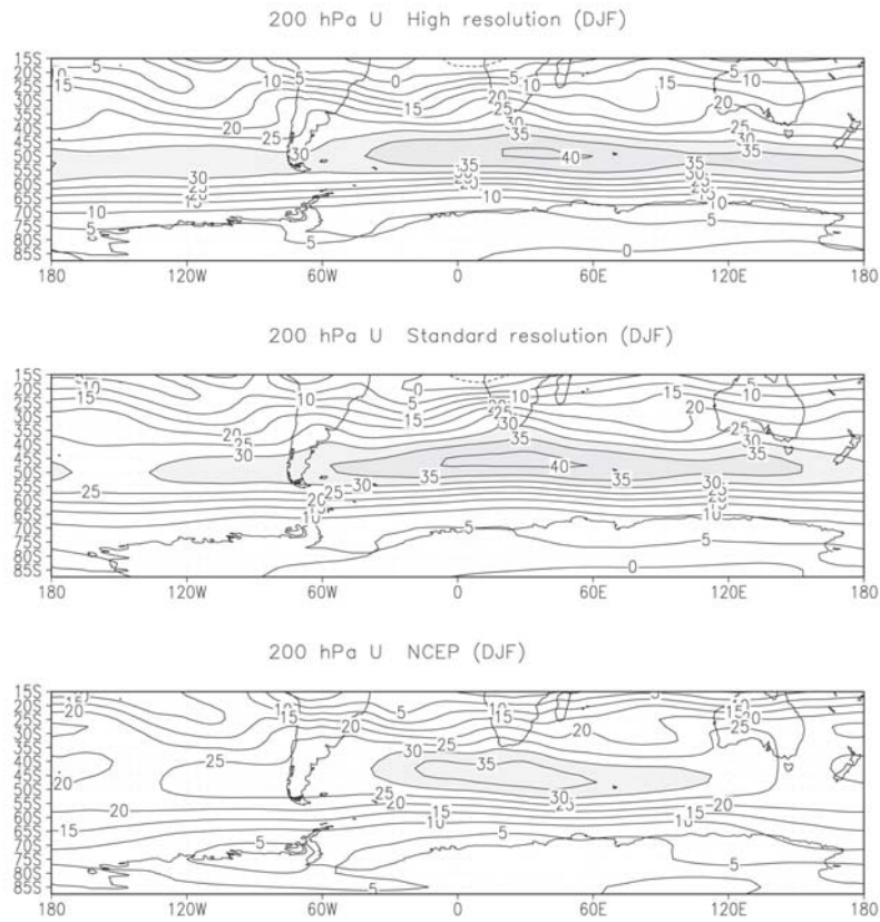
Fig. 2a. Mean DJF zonal wind at 200 hPa from High resolution (top), Standard resolution (centre) and NCEP climatology (bottom). Contours every 5 m s -1 with values larger than 30 m s -1 shaded.
