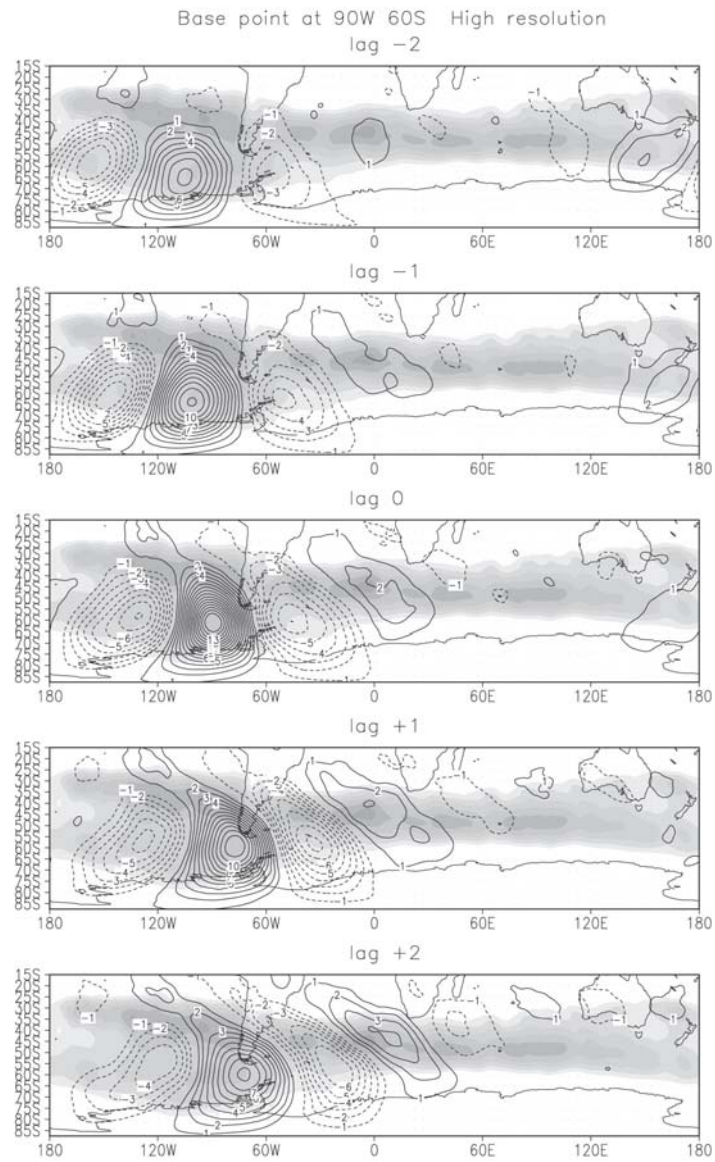
Fig. 6a. Regression for the meridional component of the wind at 200 hPa with a base point at 60° S, 90° W from lag -2 to 2 for High resolution. Contours every 1 m s -1 , zero contour is omitted. The shaded area represents the variance of meridional wind at 200 hPa larger than 180 m 2 s -2 .
