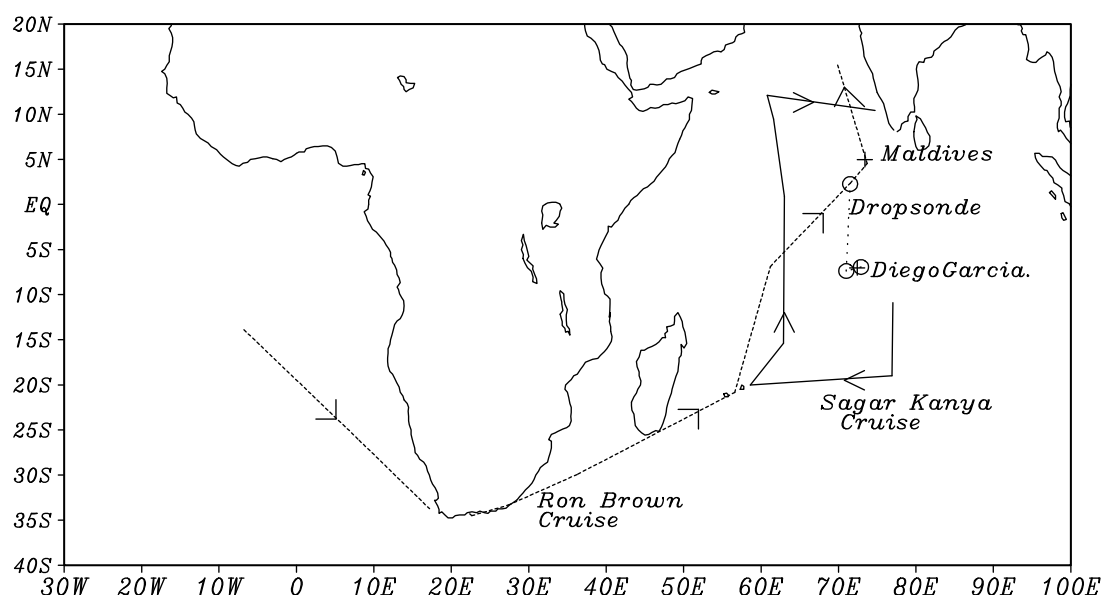
Fig. 3. Geographical location of different types of observations during INDOEX-IPF 99 (1st February-10th March 1999)
