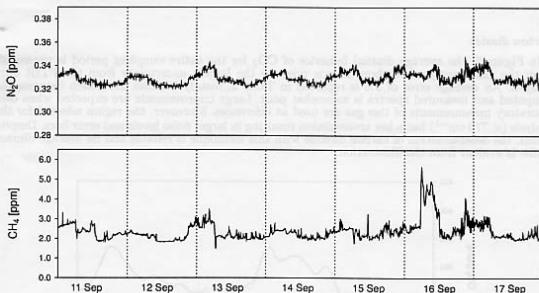
Fig. 6. N_2O and CH_4 concentration curves for September 2001 measured with the FTIR and multi-pass White cell ( \sim 23 m). Dotted lines correspond to midnight hours.
