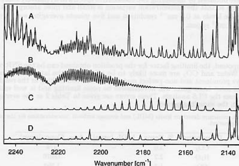
Fig. 3. FTIR spectral window showing: A one sample spectrum and B \text{N}_2\text{O} , C CO and D \text{H}_2\text{O} reference spectra computed with E-Trans.
