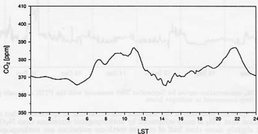
Fig. 7. Hourly \text{CO}_2 concentration at UNAM as an average of the two week period between the 11 th and the 29 th of September, 2001.
