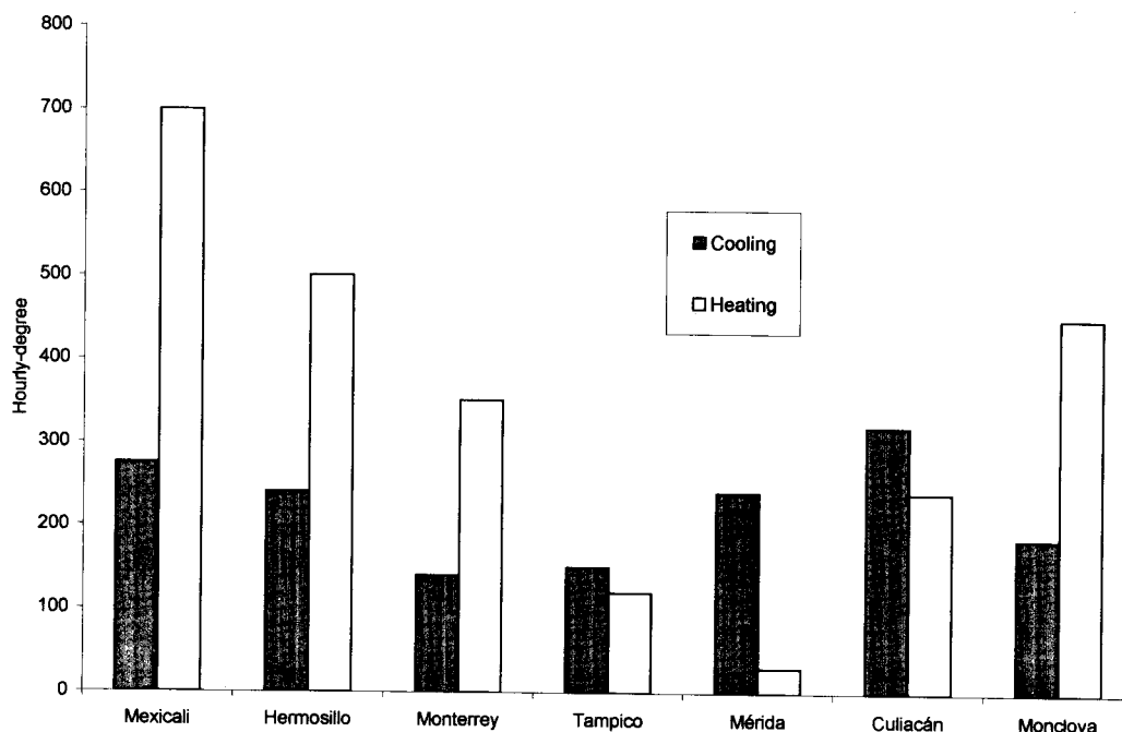
Fig. 2. Yearly needs of heating and cooling according to Thom's index.
