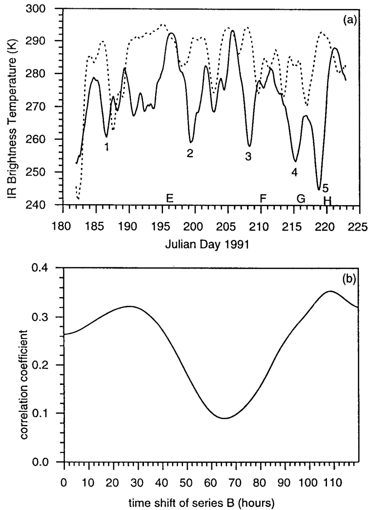
Fig. 2. (a) Time series of areal-averaged IR brightness temperature (K) for region A (solid) and region B (dashed) defined in Figure 1. The letters indicate the dates of formation of hurricanes Enrique, Fefa, Guillermo, and Hilda. (b) Linear correlation coefficient of times series as a function of forward displacement of series in Region B.
