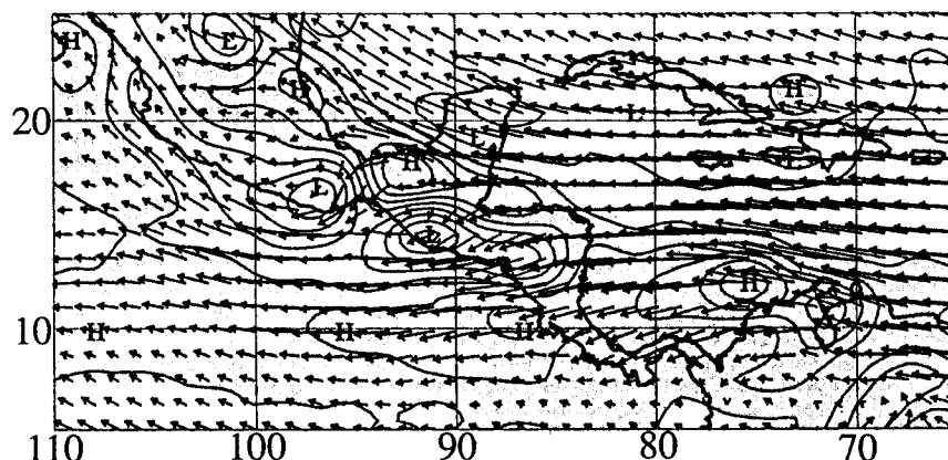
Fig. 3. Average wind and relative vorticity at 850-mb level for the period 1 July - 15 August 1991. Maximum wind vector is 15 \text{ ms}^{-1} , and relative vorticity contours are 1 \times 10^{-5} \text{ s}^{-1} . Shaded regions indicate cyclonic relative vorticity.
