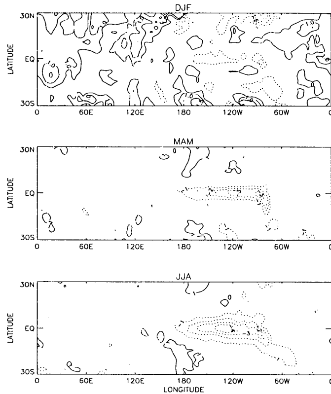
Fig. 1. SST ( ^{\circ}\text{C} ) difference between 1988 and 1987 for DJF (1a), MAM (1b) and JJA (1c). Isopleth spacing is .5^{\circ}\text{C} for DJF and 1^{\circ}\text{C} for MAM and JJA. Broken lines indicate negative values.
