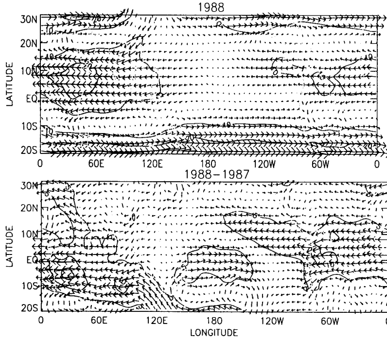
Fig. 11. Modeled(E2) JJA wind for 1988 (11a) and 1988 minus 1987 (11b) respectively. Contours of wind speed are overplotted with contour interval 10 \text{ ms}^{-1} for 1988 and 5 \text{ ms}^{-1} for 1988 minus 1987.
