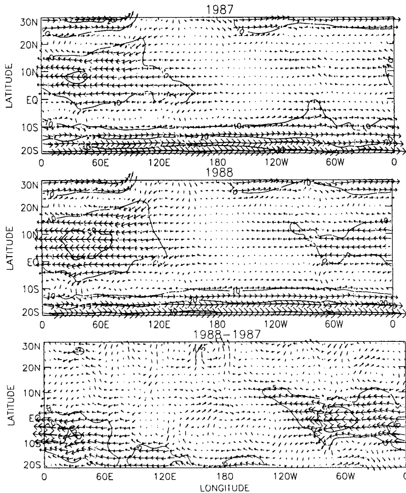
Fig. 4. Modeled JJA wind for 1987 (4a), 1988 (4b) and 1988 minus 1987 (4c) respectively. Contours of wind speed are overplotted with contour interval 10 \text{ ms}^{-1} for Figures 4a and 4b and 5 \text{ ms}^{-1} for Figure 4c.
