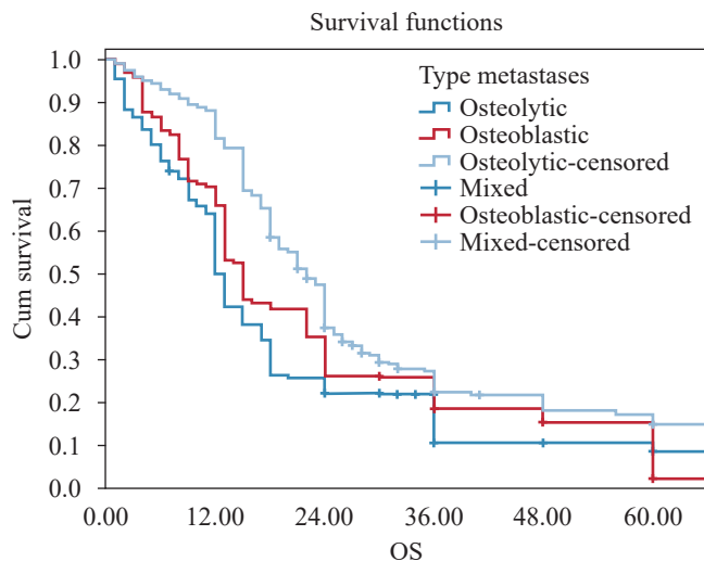
Figure 3: Overall survival and biological behavior of metastatic cancer to bone.
