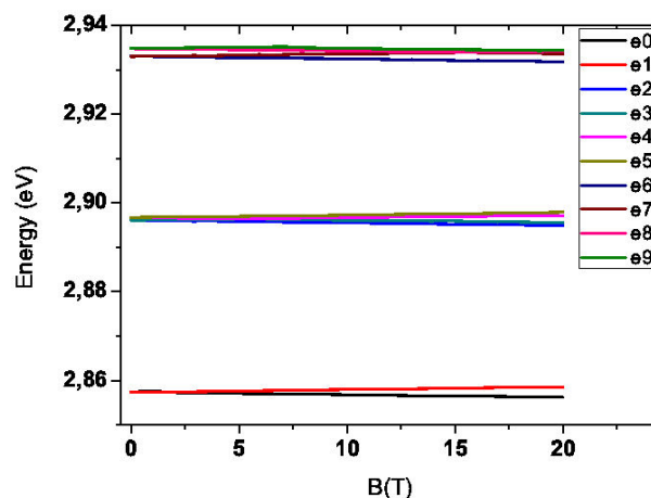
FIGURE 6. Carrier energy of electrons for the first 10 states of GaN/AlN QD's varying the magnetic field B . Strong confinement by the piezoelectric potential is also observed.
