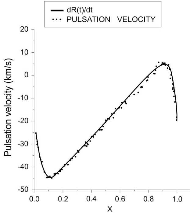
FIGURE 2. Pulsation velocity curve of \delta Cep as function of a normalized period x .
