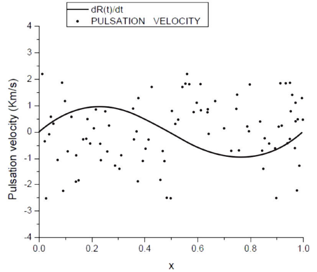
FIGURE 3. Pulsation velocity curve of Polaris as function of a normalized period x .
