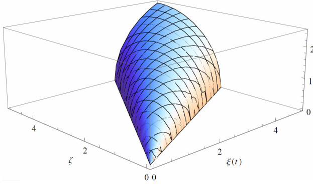
FIGURE 1. Graphics of the Function F(\xi, \zeta) .
