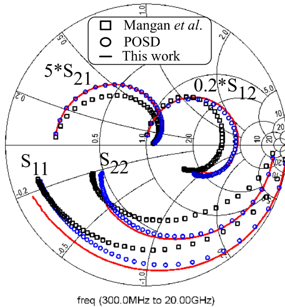
FIGURE 6. CMOS FET de-embedded at V_{GS} = 2.8 V and V_{DS} = 4.8 V using [4], PSOD and the proposed method.
