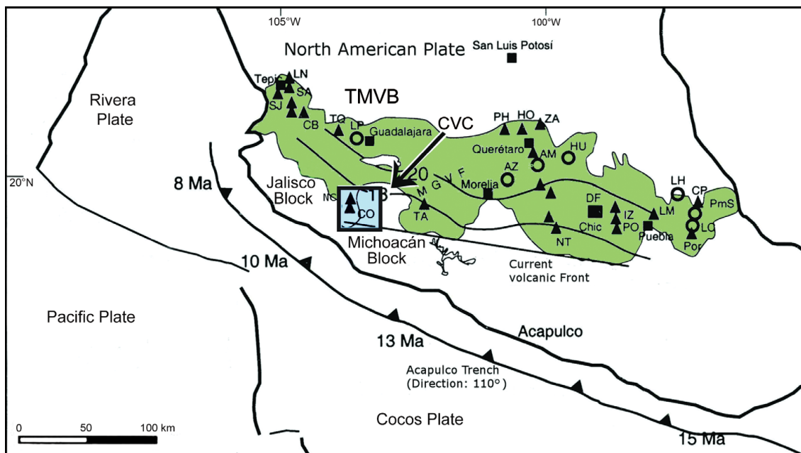
Figure 1. Location of the Trans-Mexican Volcanic Belt (TMVB, green area). Tectonic environment and principal volcanic centers of the TMVB. The blue box represents the area covered by the Colima volcanic complex (CVC) with its two main structures, Nevado de Colima and Colima volcano. Numbers at the trench refer to the age of the plate entering the subduction zone. Triangles indicate the main stratovolcanoes of the TMVB: The Navajas (LN); Sangagüey (SA); San Juan (SJ); Ceboruco (CB); Tequila (TQ); Volcano Colima (VC); Tancitaro (TA); Palo Huérano (PH); La Joya (HO); El Zamorano (ZA); Nevado de Toluca (NT); Iztaccihuatl (IZ); Popocatepetl (PO); La Malinche (LM); Cofre de Perote (CP); Pico de Orizaba (Por). The circles indicate volcanic calderas: La Primavera (LP); Los Azufres (AL); Amealco (AM); Huichapan (HU); Los Hornos (LH); MGVF is one of the principal volcanic fields: Michoacán-Guanajuato volcanic field; Chic is the Sierra de Chichinautzin; Pms Chiconquaco-Palma Sola.
