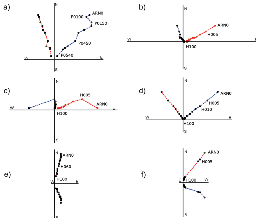
Figure 4. Examples of orthogonal vector plots, showing thermal demagnetization since ARN0 with steps of 50^\circ\text{C} until 540^\circ (label with an initial “P” example P0540) for the alternating field demagnetization since ARN0 with steps of demagnetization 5 mT until 100 mT (label with an initial “H” example H100). a) Sample 94C026A corresponding to the site Col3. b) Sample 94C001A, site Col1. c) Sample 94C011B, site Col2. d) Sample 94C035A, site Col4, including two orthogonal vector plots of events belonging to transitional geomagnetic regime. e) Sample 94C062A, site Col8. f) Sample 94C098A, site Col10.
