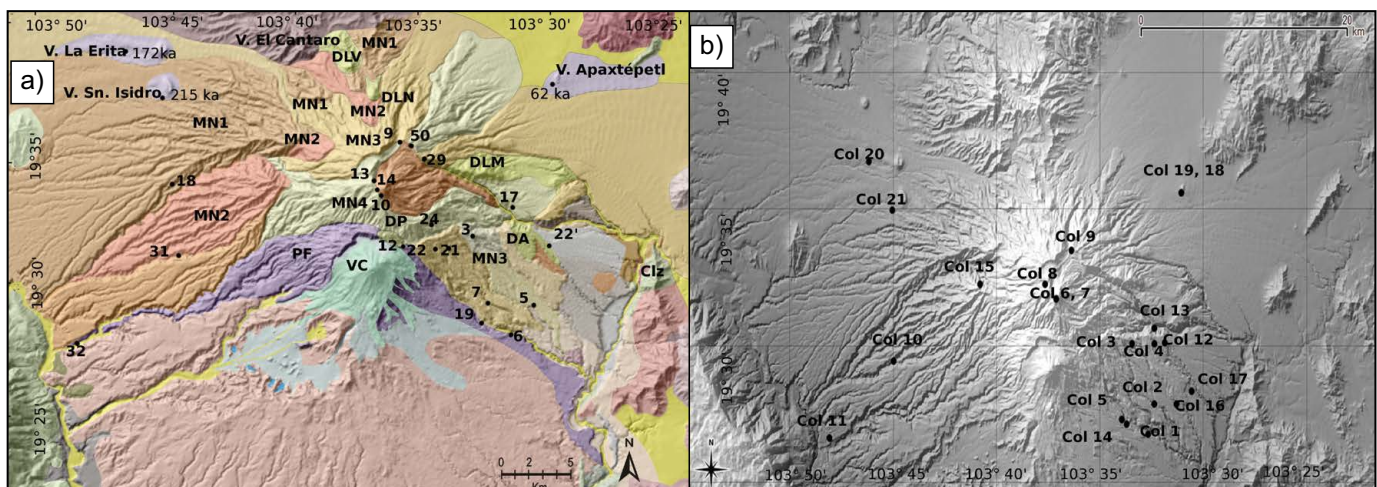
Figure 2. Geological map of the Colima volcanic complex area showing sample site locations. a) All 30 available radiometric dates from the area (Córtes et al. , 2015). b) Location of the 21 paleomagnetic sites for this study.
