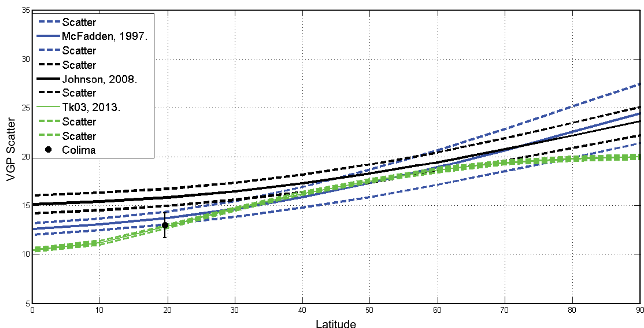
Figure 7. Scatter of the VGP as function of the latitude for the last 5 Myr, compared with the model G of McElhinny and McFadden (1997) (blue line labelled McFadden, 1997), Johnson et al. (2008) (black line labelled Johnson, 2008) and the Tk03 model proposed by Tauxe and Kent (2013) (green line).
