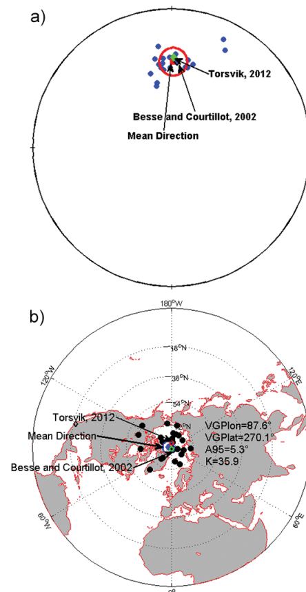
Figure 6. a) Equal area projection of the mean paleomagnetic directions obtained in this study; b) projection of the VGPs together with reference paleomagnetic poles recalculated from the stable North America (Besse and Courtillot, 2002; Torsvik et al. , 2012).
