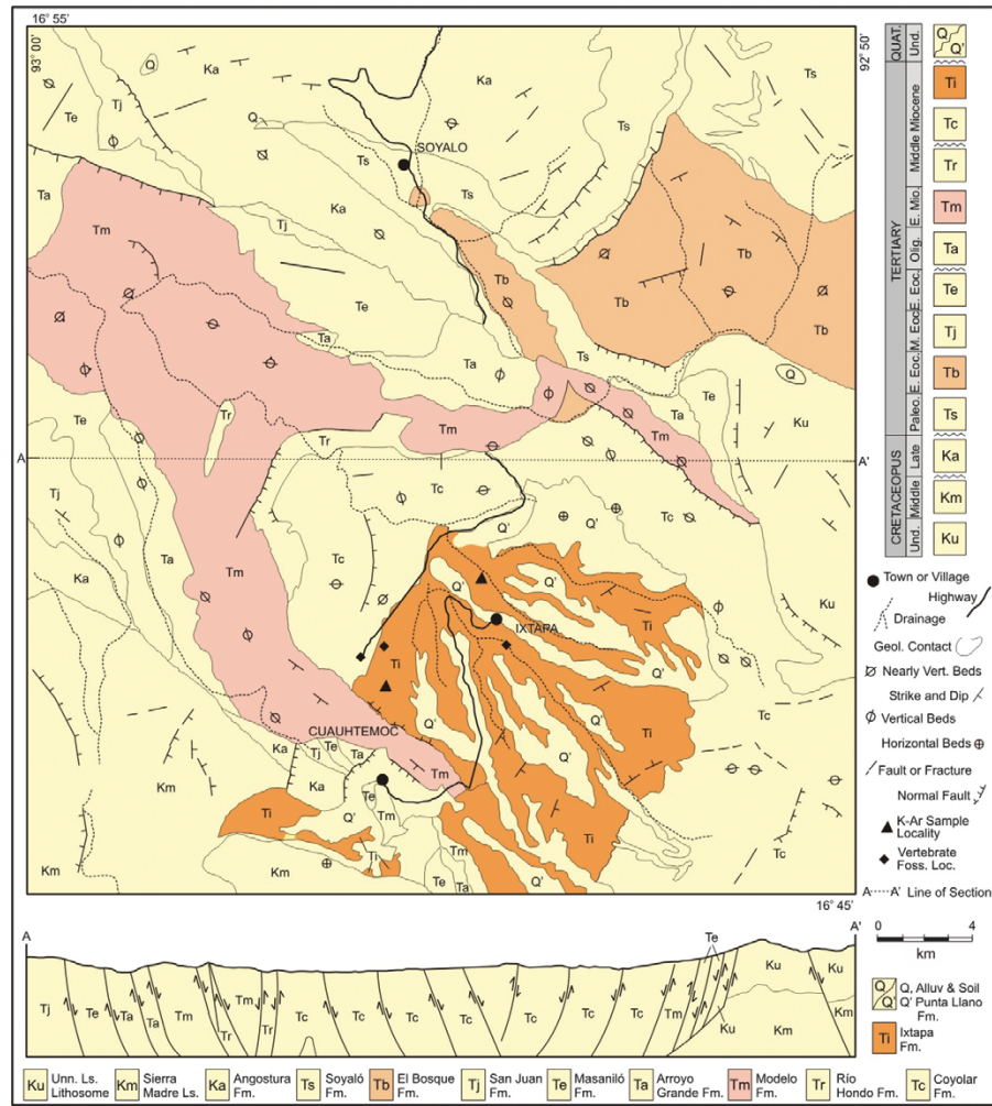
Figure A9. Geologic map of the Ixtapa Site (taken from Ferrusquía-Villafranca, 1996).
