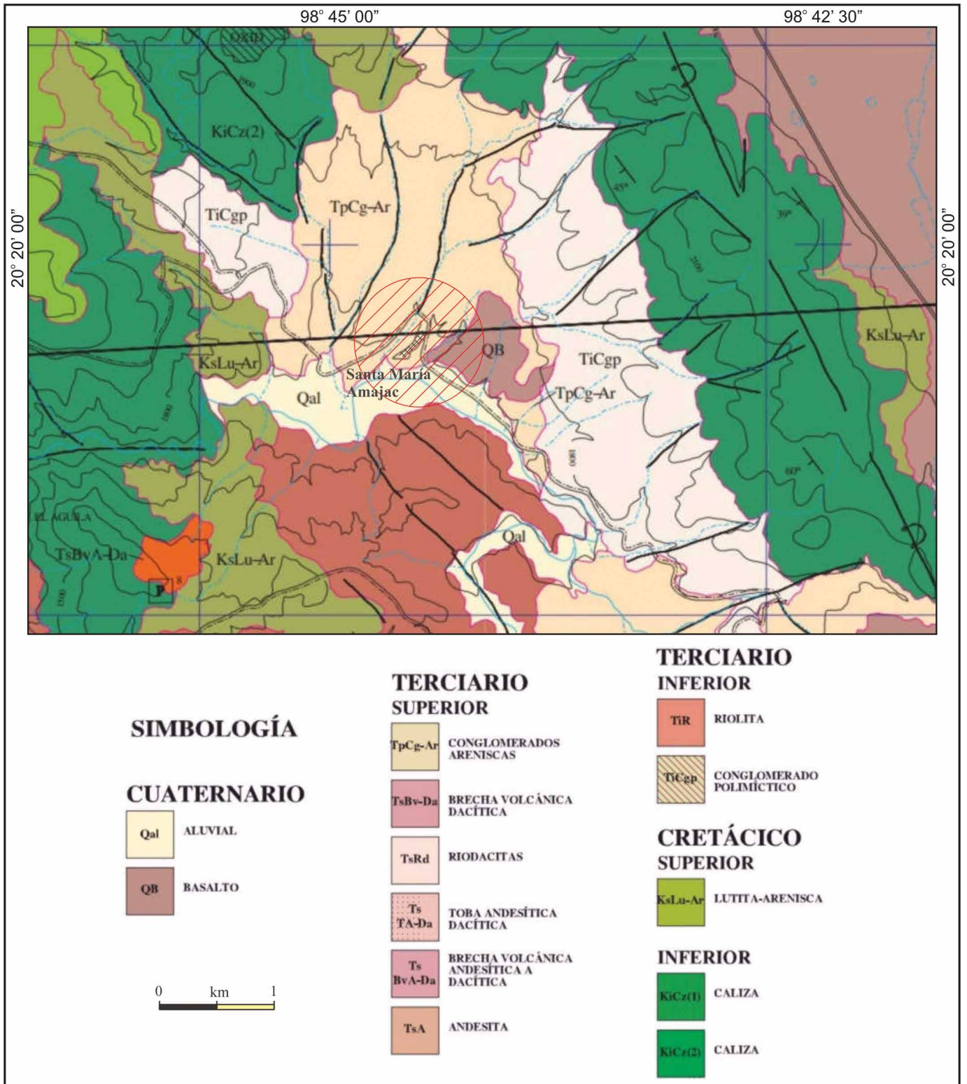
Figure A18. Geologic map of the Santa María Amajac Site (taken and slightly edited from SGM, 1995a).
