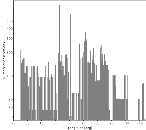
Fig. 1. Number of observations for each observing window corresponding to objects in the interval 8.6^\circ \text{W} < \lambda < 117.5^\circ \text{W} and -0.165 < \delta < 0.165 . The available number of observations allows the determination of the relative motion of orbiters in the GEO ring over different time scales.
