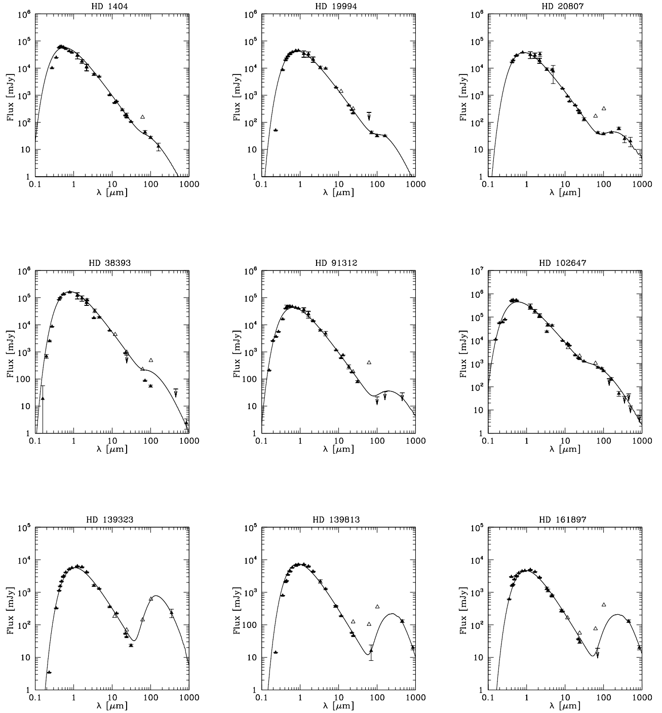
Fig. 5. Model SEDs for the sample of binary stars. Triangles indicate actual fluxes and arrows upper limits. Error bars for fluxes at different wavelengths are included. Observations from IRAS are indicated with empty triangles but were not used in the modeling.
